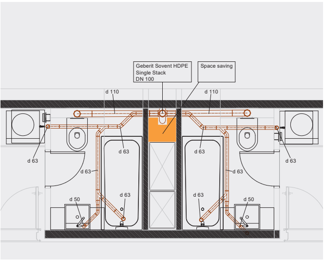
Final plan with Geberit Sovent
